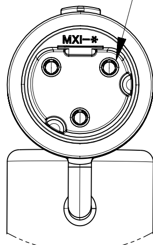
VIEW SHOWING KEYING OF 3 CIRCUIT VERSION
