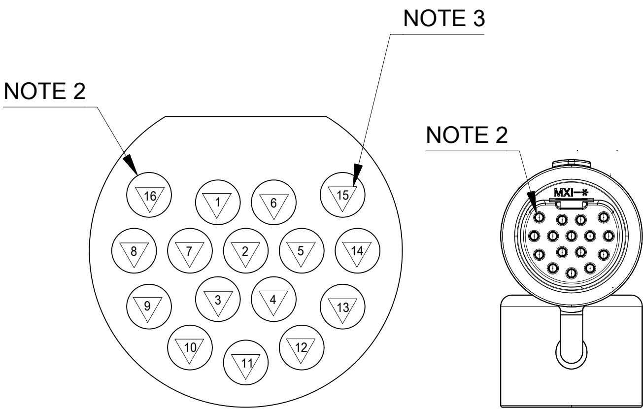
16 CIRCUIT WIRE LAYOUT CONNECTOR FRONT VIEW
