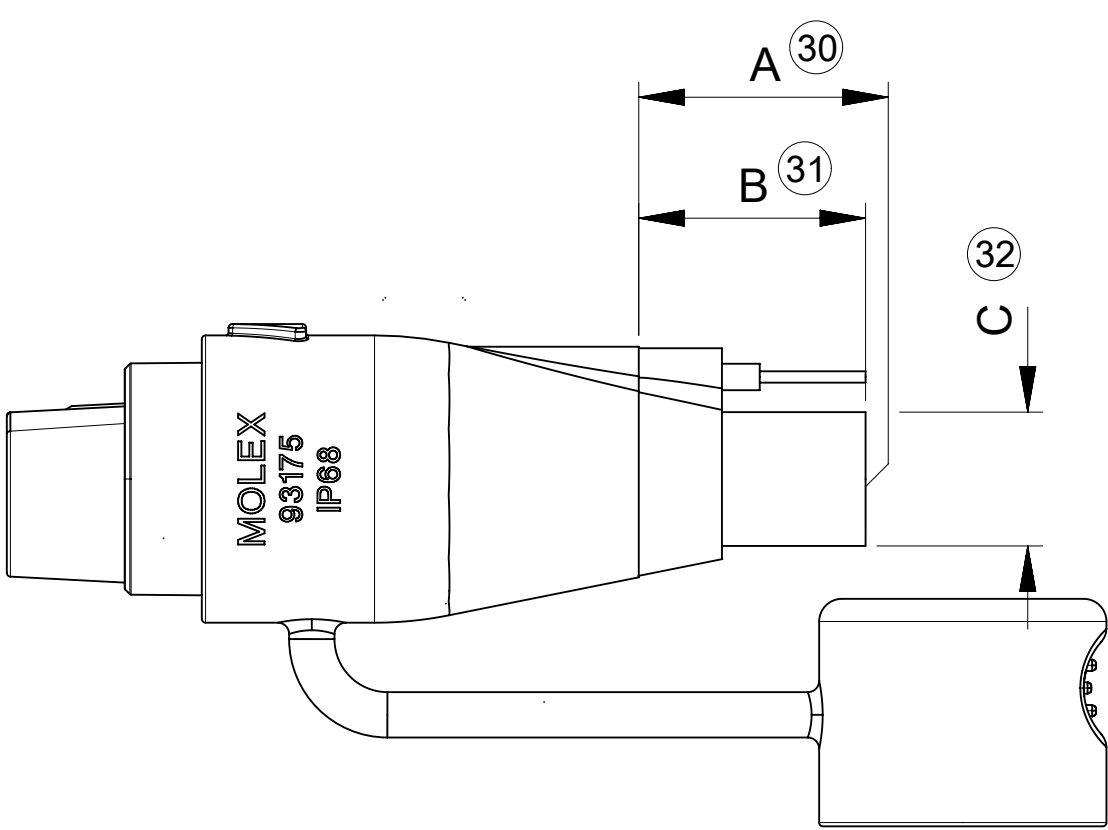
FEMALE POLE PLUG CONNECTOR 16 CIRCUIT
