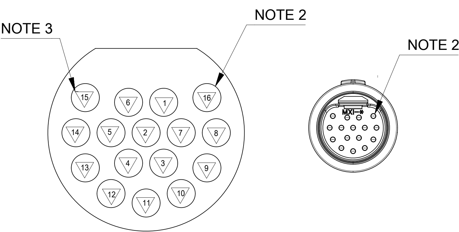
16 CIRCUIT WIRE LAYOUT CONNECTOR FRONT VIEW
