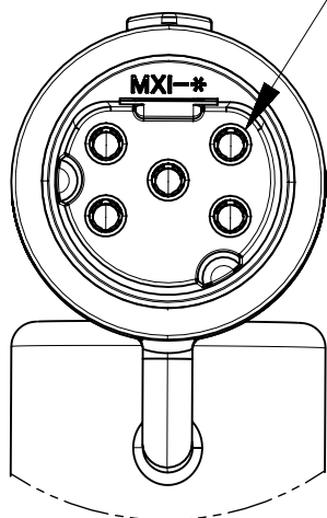
VIEW SHOWING KEYING OF 5 CIRCUIT VERSION
