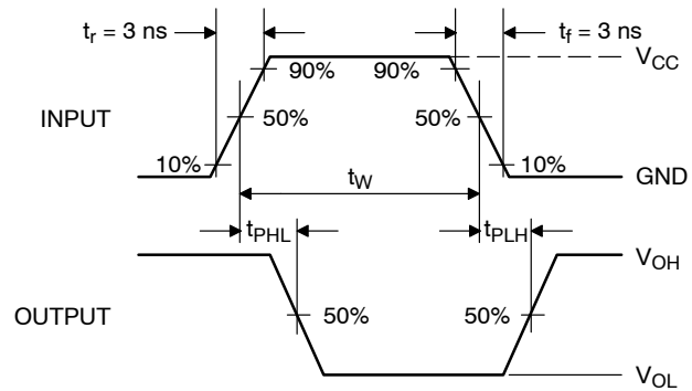
Figure 6. AC Waveforms
