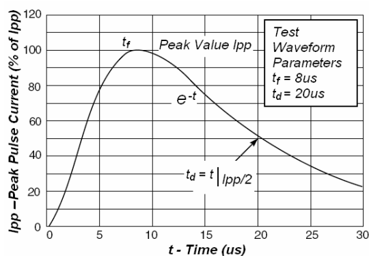
Fig 1. Pulse Waveform
