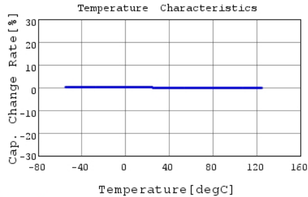
GRM0335C1E7R2CA01 C-Temp. capchange, DCOV, 1
