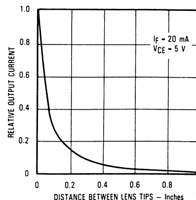
Coupling Characteristics of OP169 and OP509
