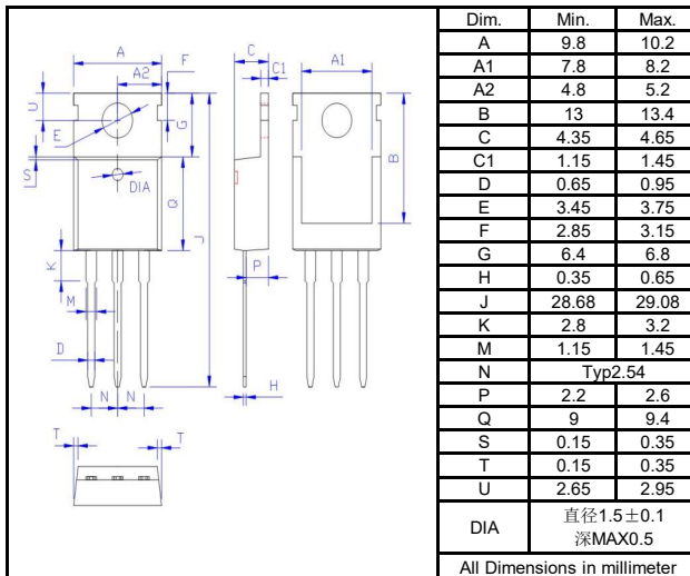
T0-220C
