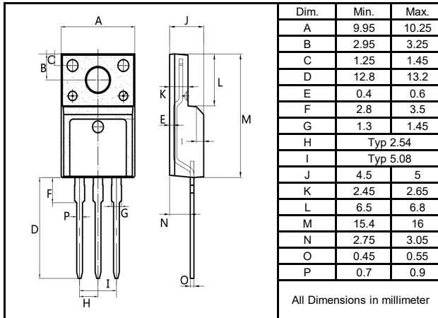
T0-220F
