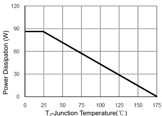
Figure 9 Power De-rating
