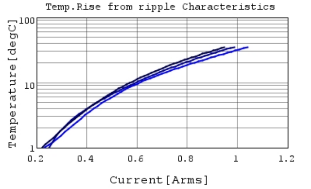
GQM2195G2E3R9CB12 Temp.rise 1GHz 2
