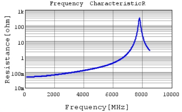
GQM2195G2E3R9CB12 R DC0V, 25degC
