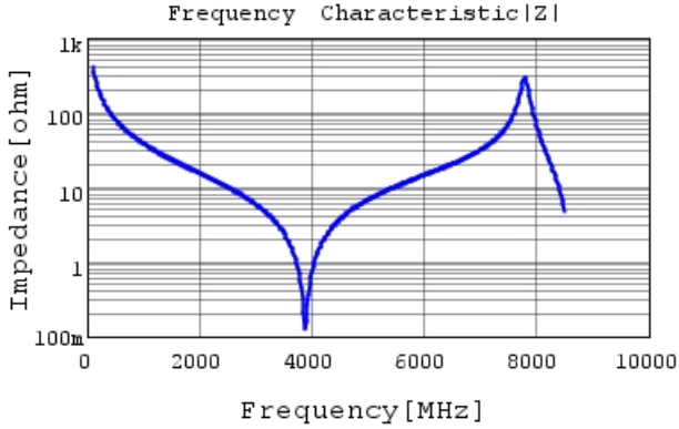
GQM2195G2E3R9CB12 |Z| DC0V, 25degC
