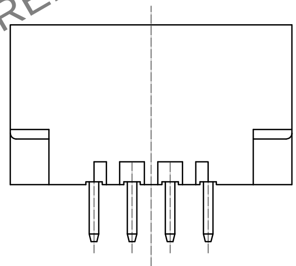
MATING FIGURE (2:1)
