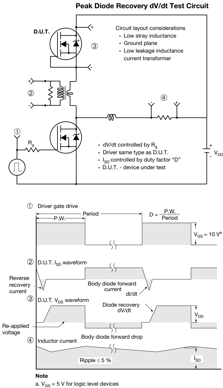
Fig. 19 - For N-Channel
