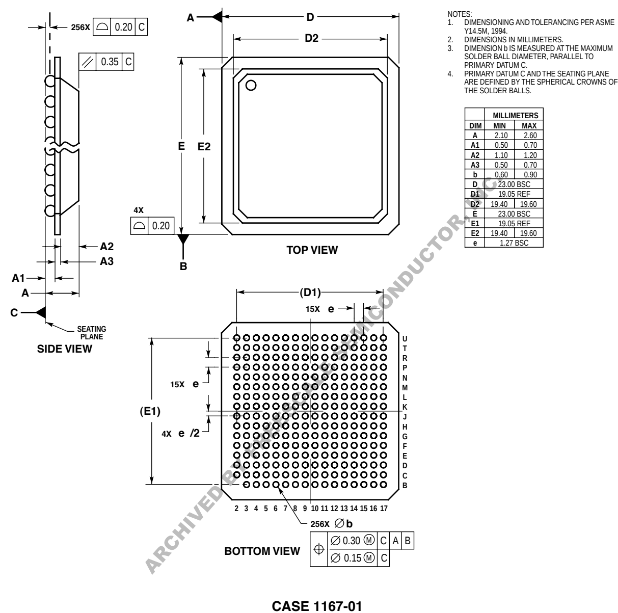
Figure 12. Package Dimensions for the Plastic Ball Grid Array (PBGA)—JEDEC Standard
