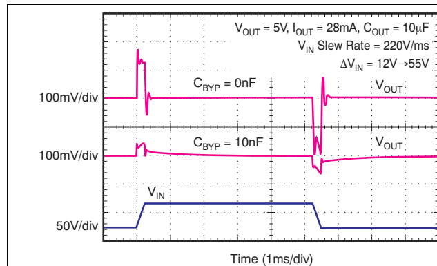
Figure 15. Line Transient Response vs C_{BYP}
