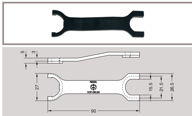
COP.155.GN Spanner for rear nut
