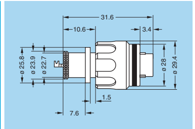
FG●.LM.U2A.XPAT Straight plug, key (W) or key (R) with arctic grip and mold stop
