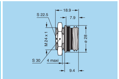
EG●.LM.U2A.XPL Fixed socket, nut fixing, key (W) or key (R)
