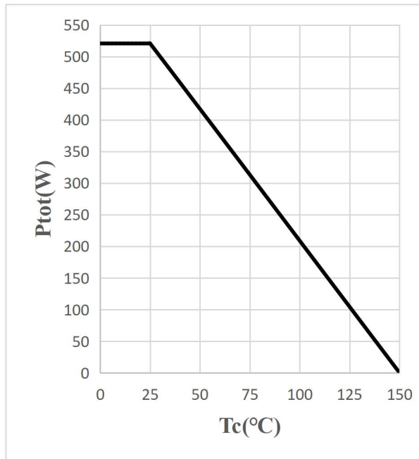
Figure 3: Power Dissipation
