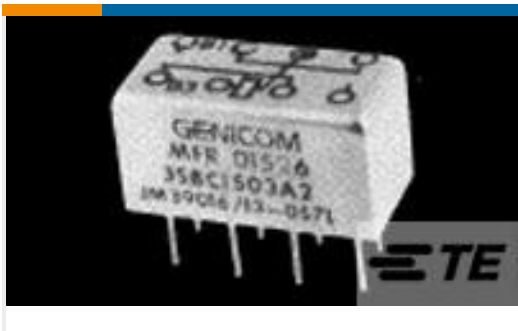
TE Part #1617074-9 3SBC5005K1 = RELAY
