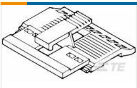
TE Part #102681-1 12 AMPMODU MT COVER DR .100CL
