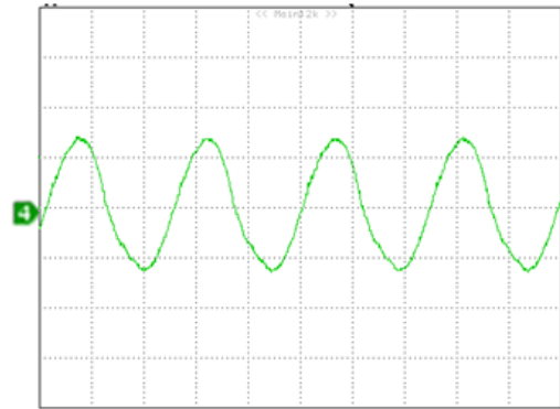
Figure 10: Input Terminal Ripple Current, i_c , at full rated output current and nominal input voltage with 12 \mu H source impedance and 33 \mu F electrolytic capacitor ( 200 \text{ mA/div} , 1 \mu s/div )
