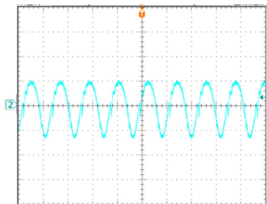
Figure 13: Output voltage ripple at nominal input voltage and rated load current ( I_o=10A ) ( 50 \text{ mV/div} , 2 \mu s/div ) Load capacitance: 1 \mu F ceramic capacitor and 10 \mu F tantalum capacitor. Bandwidth: 20 \text{ MHz} . Scope measurements should be made using a BNC cable (length shorter than 20 inches). Position the load between 51 mm to 76 mm (2 inches to 3 inches) from the module.
