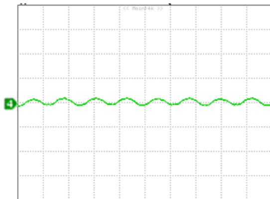
Figure 11: Input reflected ripple current, i_s , through a 12 \mu H source inductor at nominal input voltage and rated load current ( 20 \text{ mA/div} , 2 \mu s/div )
