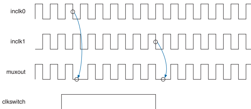
Figure 5–23. Manual Switchover
