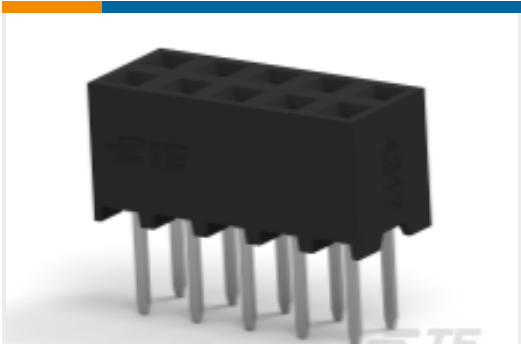
TE Part #1-2314822-0 10P,2MM,B-B,REC,DRVT,2.7,0.76AU,TB
