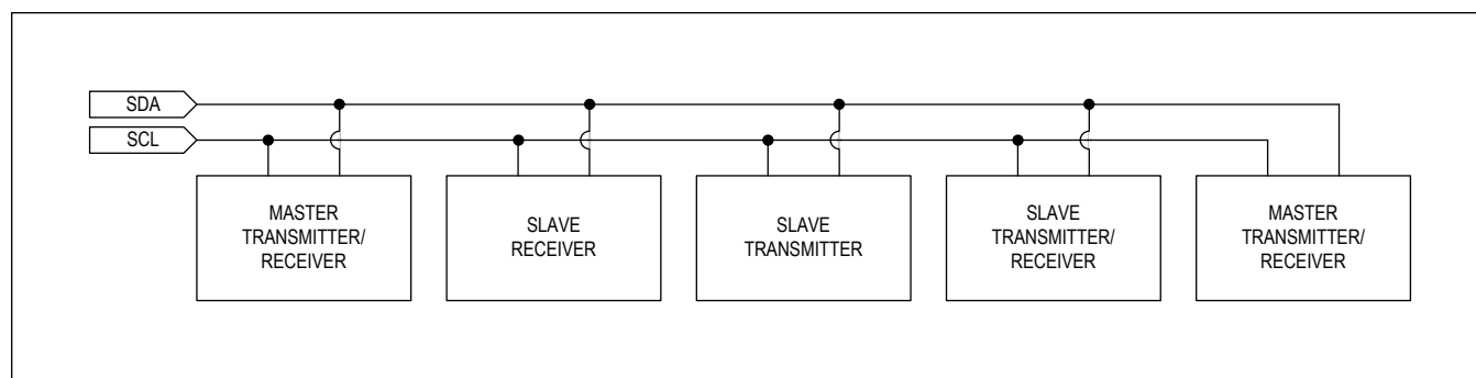
Figure 30. I 2 C System Configuration
