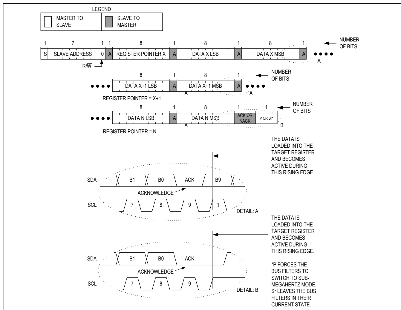
Figure 35. Writing to Sequential Registers X to N
