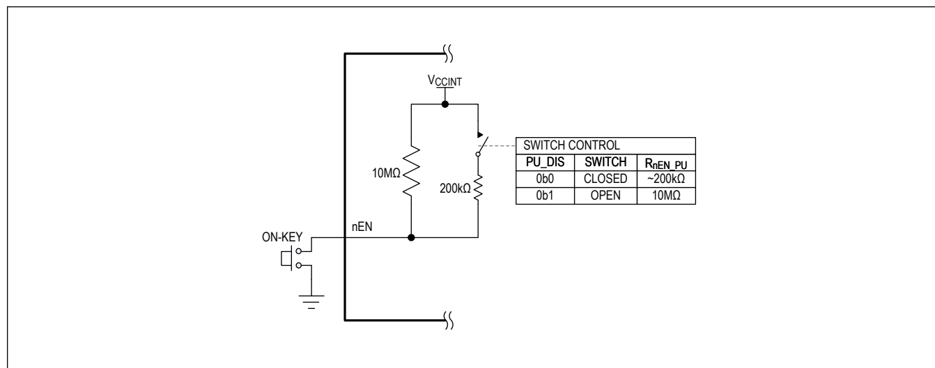
Figure 4. nEN Pullup Resistor Configuration
