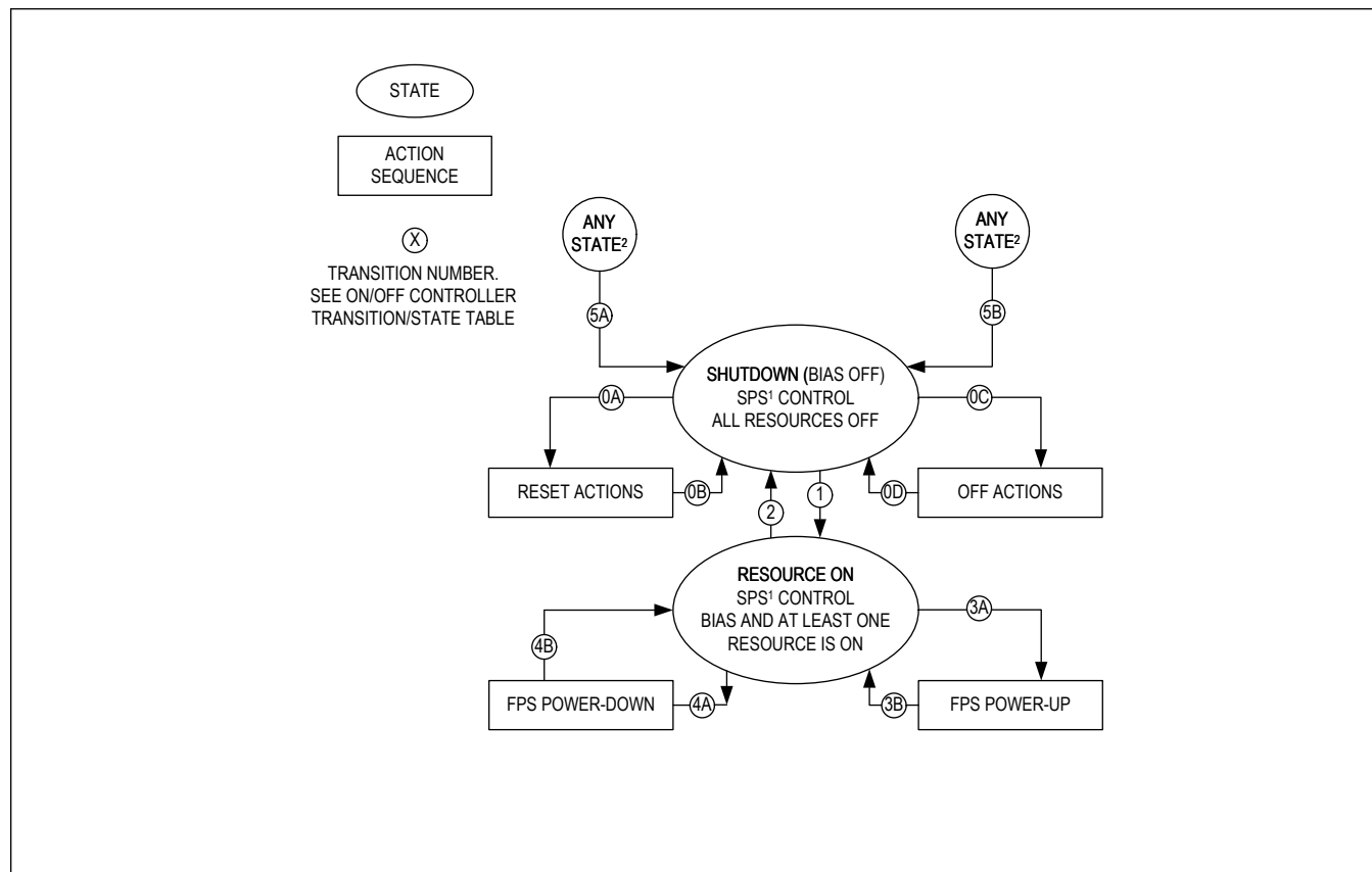
Figure 7. Top Level On/Off Controller State Diagram
