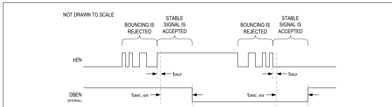
Figure 5. Debounced Input
