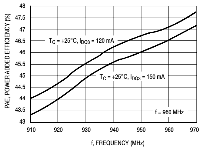
Figure 10. Power Added Efficiency versus Frequency Pout = 10 W
