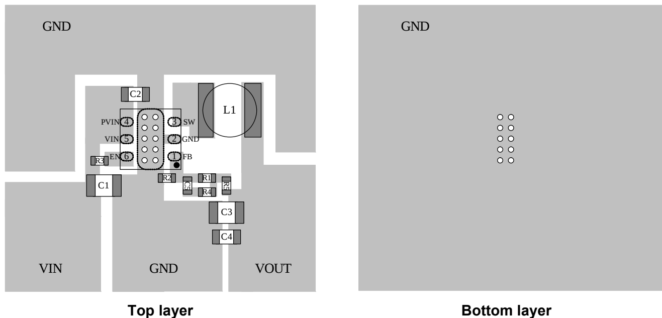
Figure 3—PCB Layout
