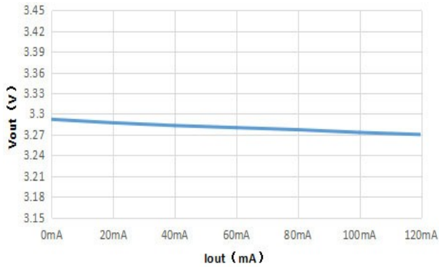
Load Regulation ( V_{in}=30\text{V} )
