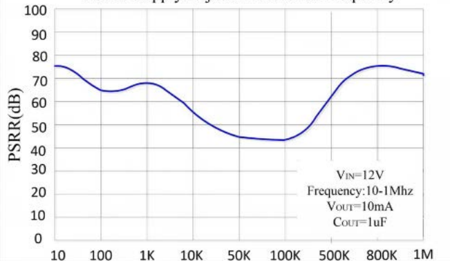
Power-Supply Rejection Ratio vs. Frequency
