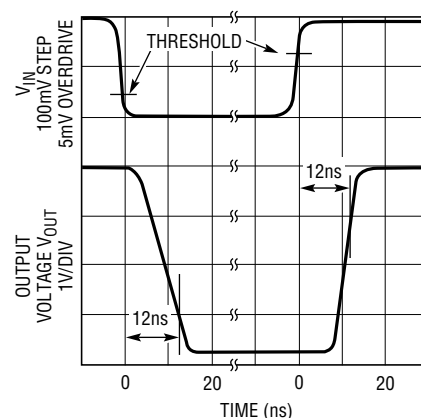
Comparator Response Time
