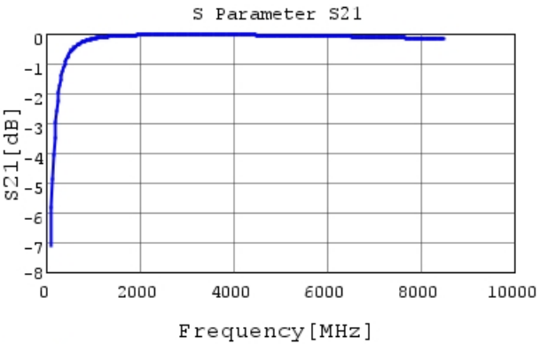
GRM0335C1H7R8CA01 S21 DCOV, 25degC
