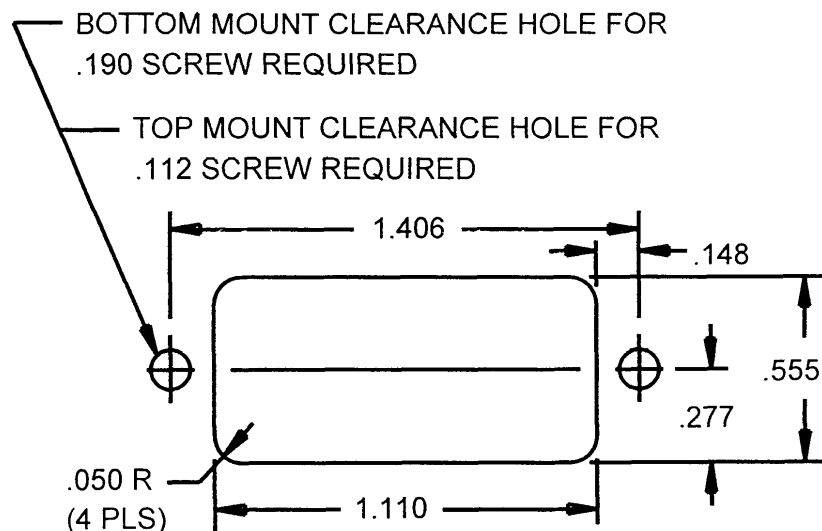
RECOMMENDED MOUNTING DIMENSIONS
