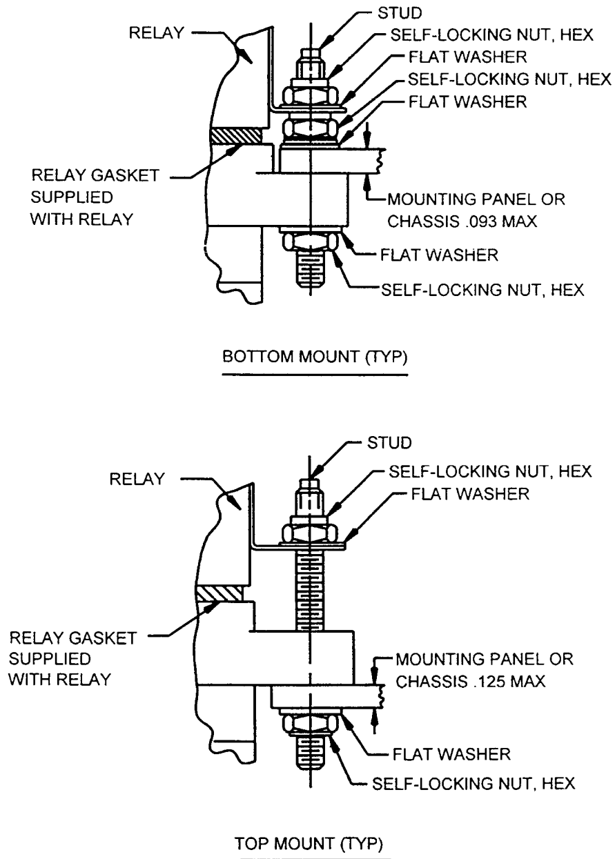
FIGURE 1. Socket configuration – Continued.
