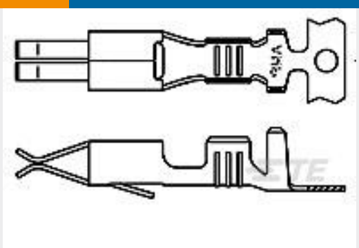
TE Part #643222-1 MINI-SPRING RECEPTACLE 20-16 AWG PTPBR
