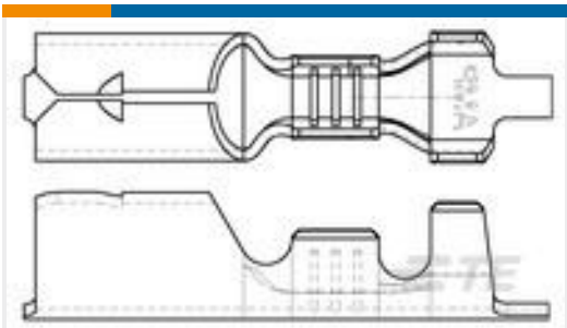
TE Part #626400-2 .156 SHUR PLUG REC.
