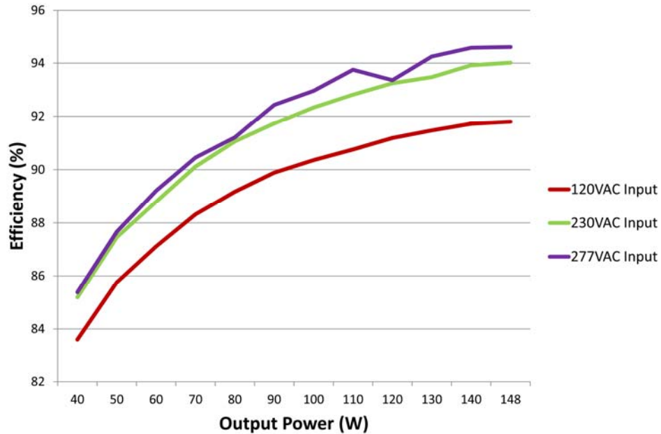
Efficiency vs Output Power
