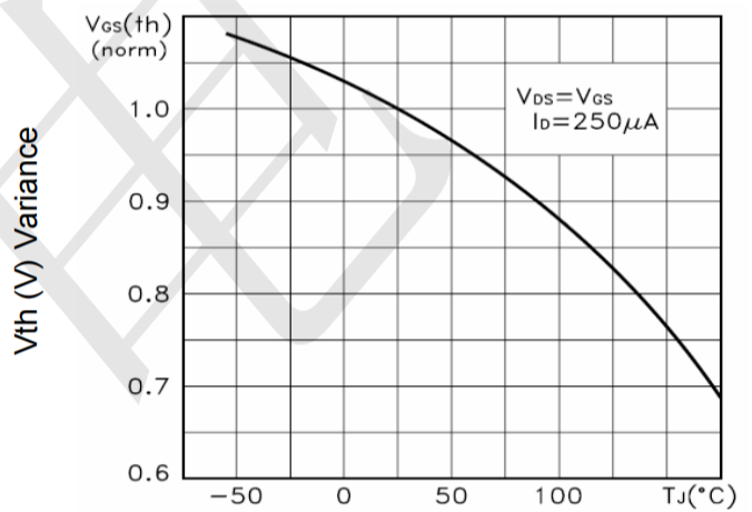
Figure 10 V GS(th) vs Junction Temperature
