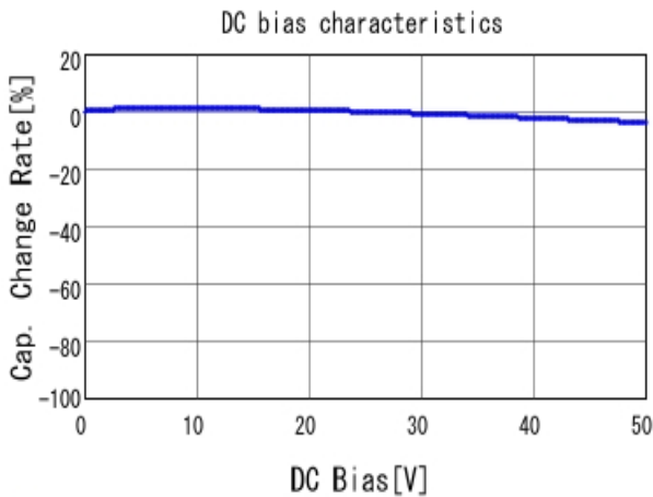
■ GRM188R11H102KA01 C-DC bias capchange, 20.0degC, AC1.
