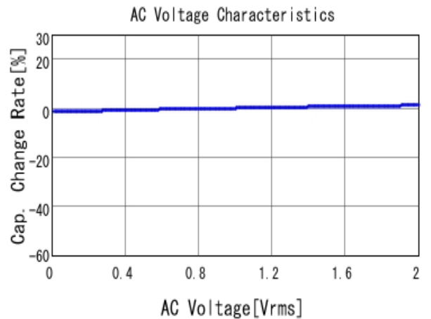
■ GRM188R11H102KA01 C-AC Voltage capchange, DC0V, 20.0d
