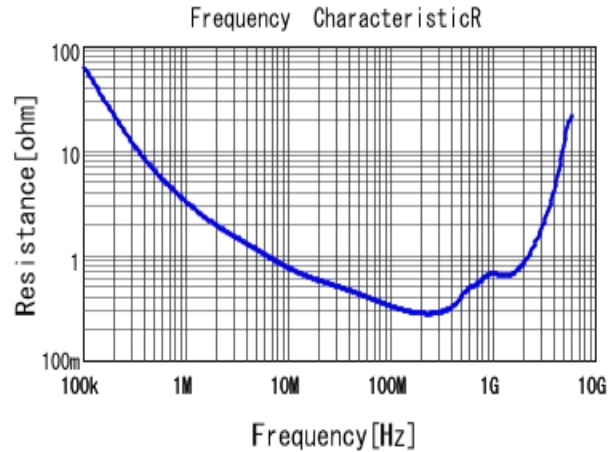
■ GRM188R11H102KA01 R DC0V, 20degC
