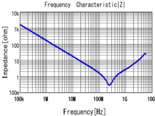
■ GRM188R11H102KA01 |Z| DC0V, 20degC
