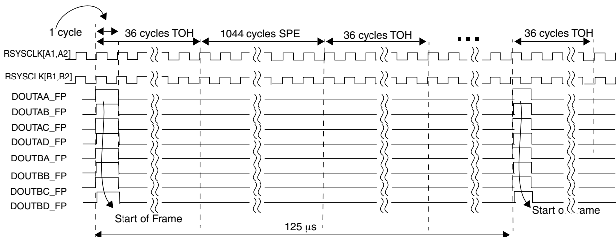
Figure 34. Receive SONET Mode—Octal Alignment Mode – ORSO82G5
