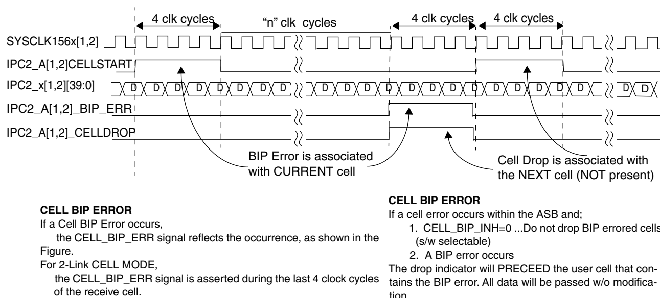
Figure 45. IPC2 Data Flow
