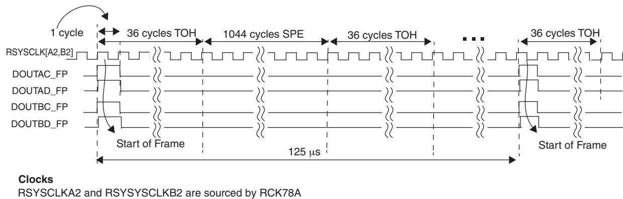
Figure 31. Receive SONET Mode, Quad Alignment Mode – ORSO42G5
