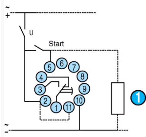
Timer 814 - 11-pin
