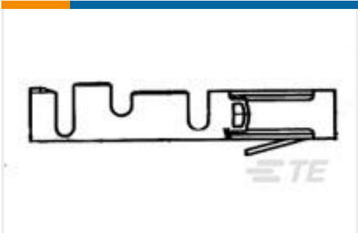
TE Part #87667-1 MOD IV RECP LP
