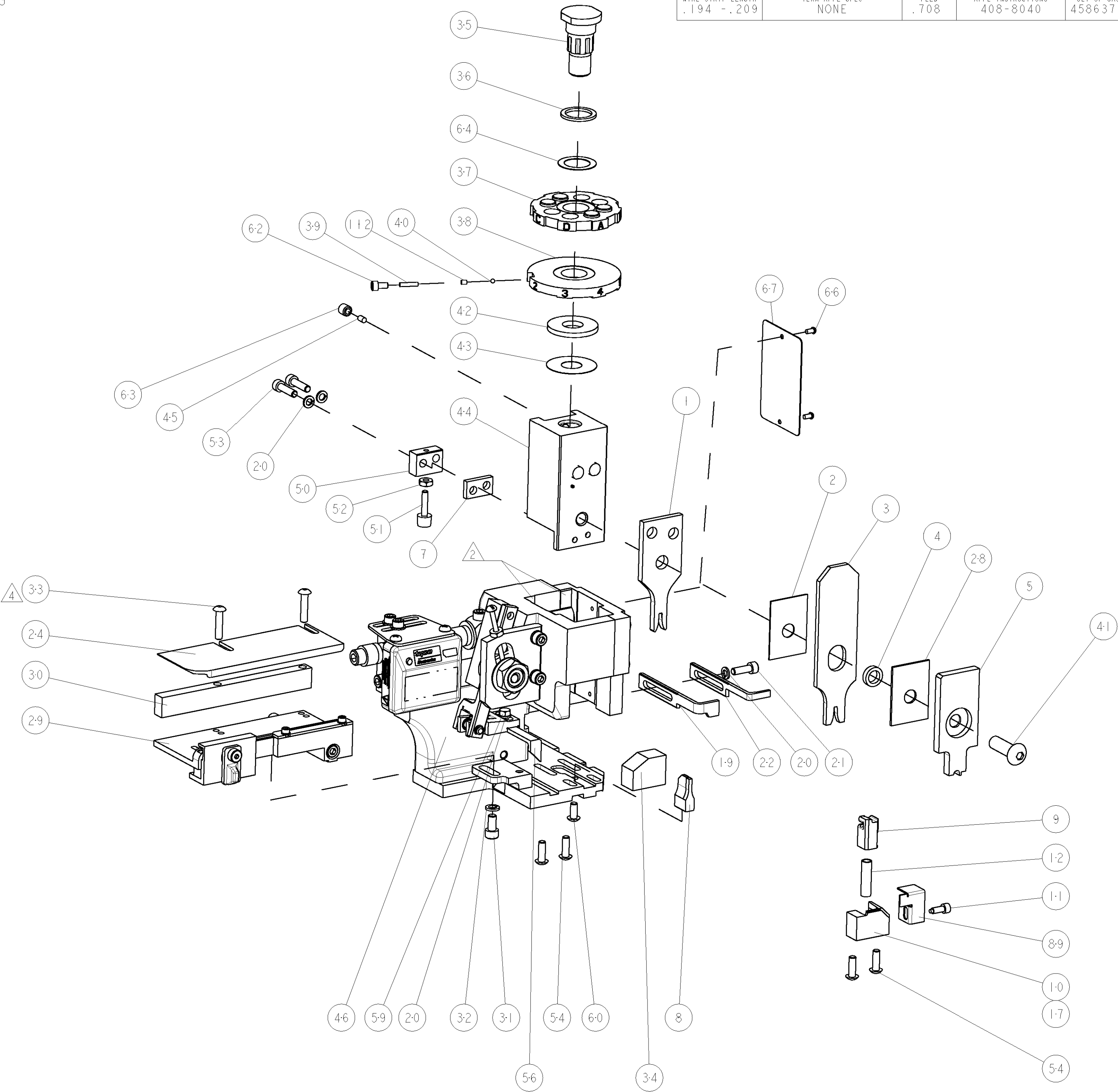
AMP-O-LECTRIC TERM GUARD G TERMINATOR GUARD
