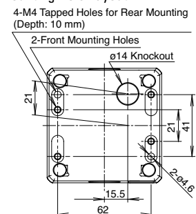
Mounting Hole Layout
