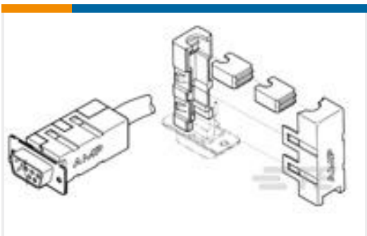
TE Part #745553-1 HDE CABLE CLAMP KIT
