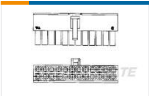
TE Part #1-1586019-2 12P RCPT VAL-U-LOK V0
