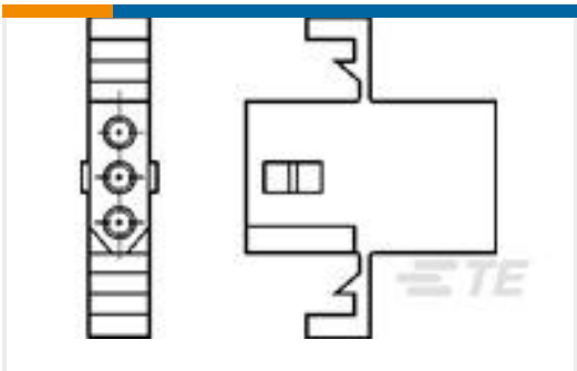
TE Part #770343-1 02P .062 COMM P&S RECPT
