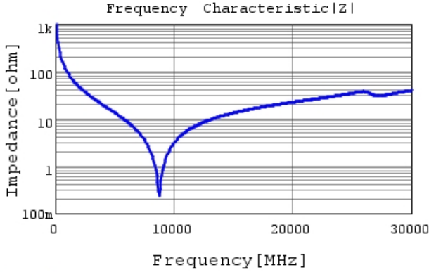
GJM0335C2A1R6WB01 |Z| DCOV, 25degC
