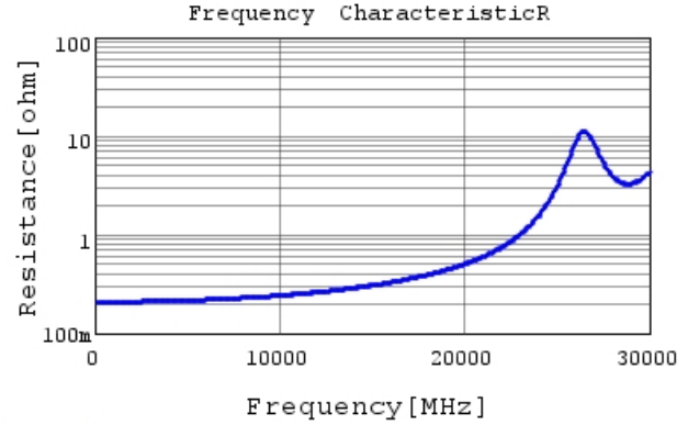
GJM0335C2A1R6WB01 R DCOV, 25degC
