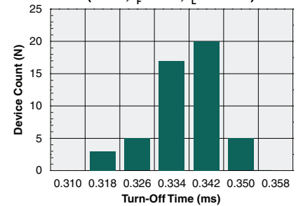
Typical Turn-Off Time (N=50, I_F=5\text{mA} , I_L=150\text{mA} )
