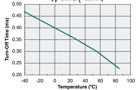
Typical Turn-Off Time vs. Temperature ( I_F=5\text{mA} , I_L=80\text{mA} )
