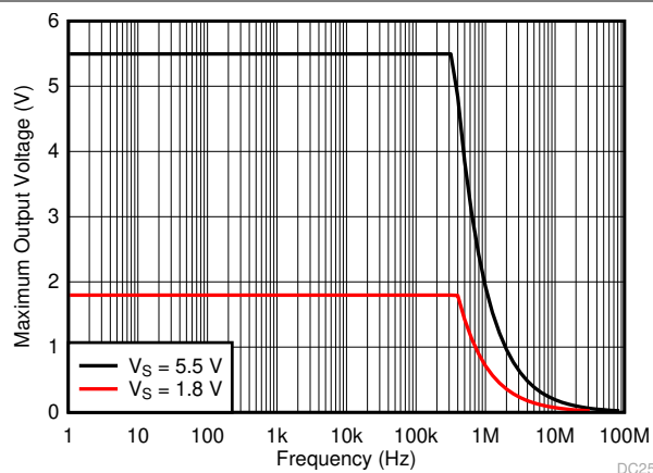
Figure 6-32. Maximum Output Voltage vs Frequency and Supply Voltage
