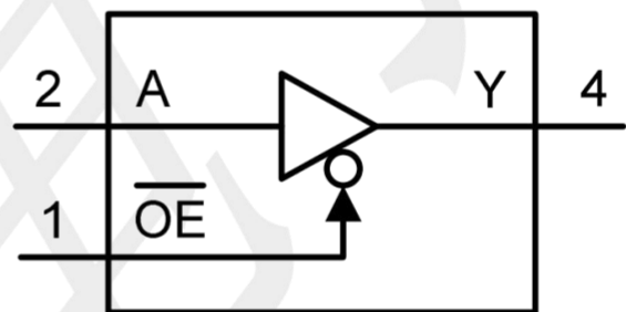
Logic Symbol
