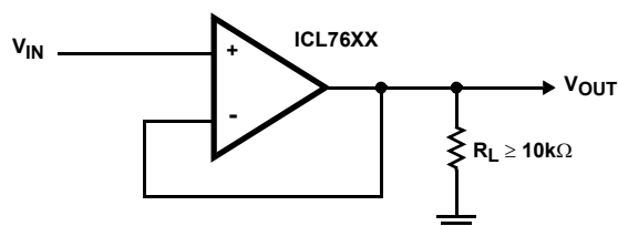
FIGURE 1. SIMPLE FOLLOWER
