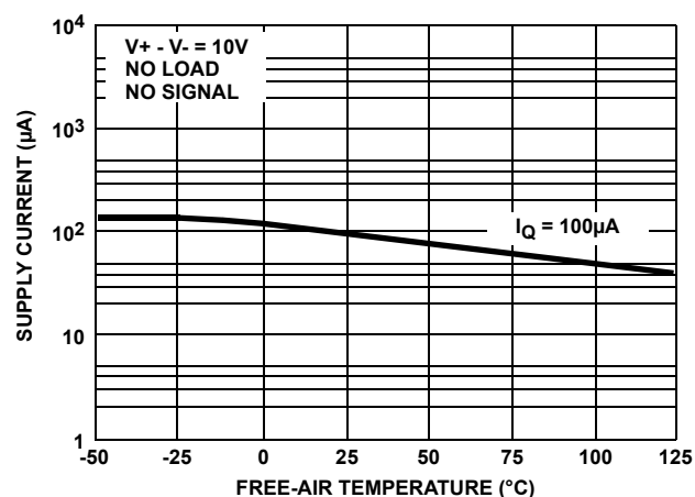
FIGURE 9. SUPPLY CURRENT PER AMPLIFIER vs FREE-AIR TEMPERATURE
