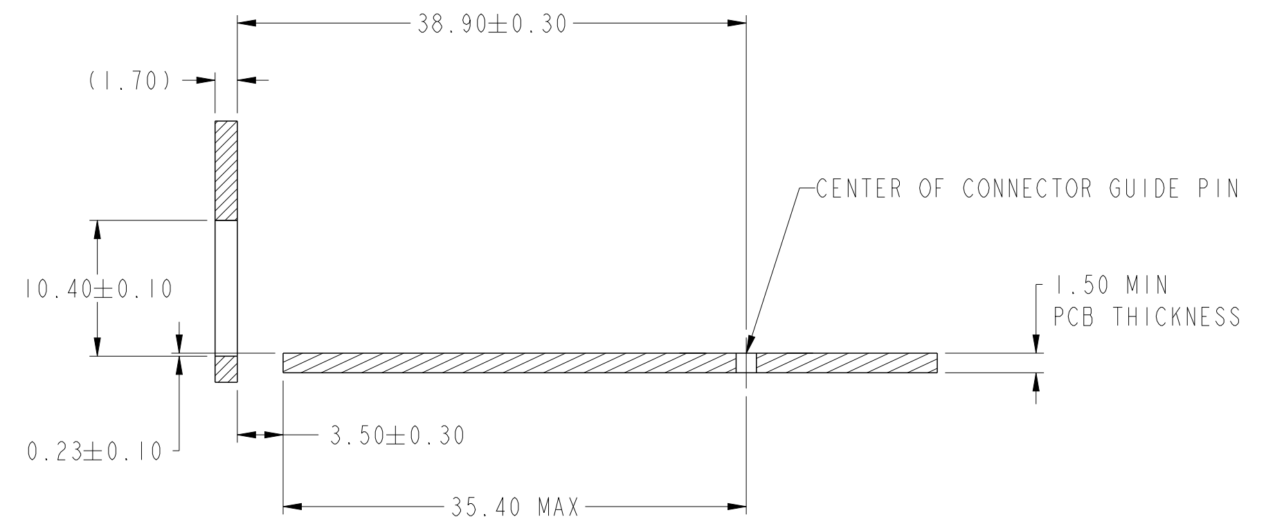
SECTION C-C
