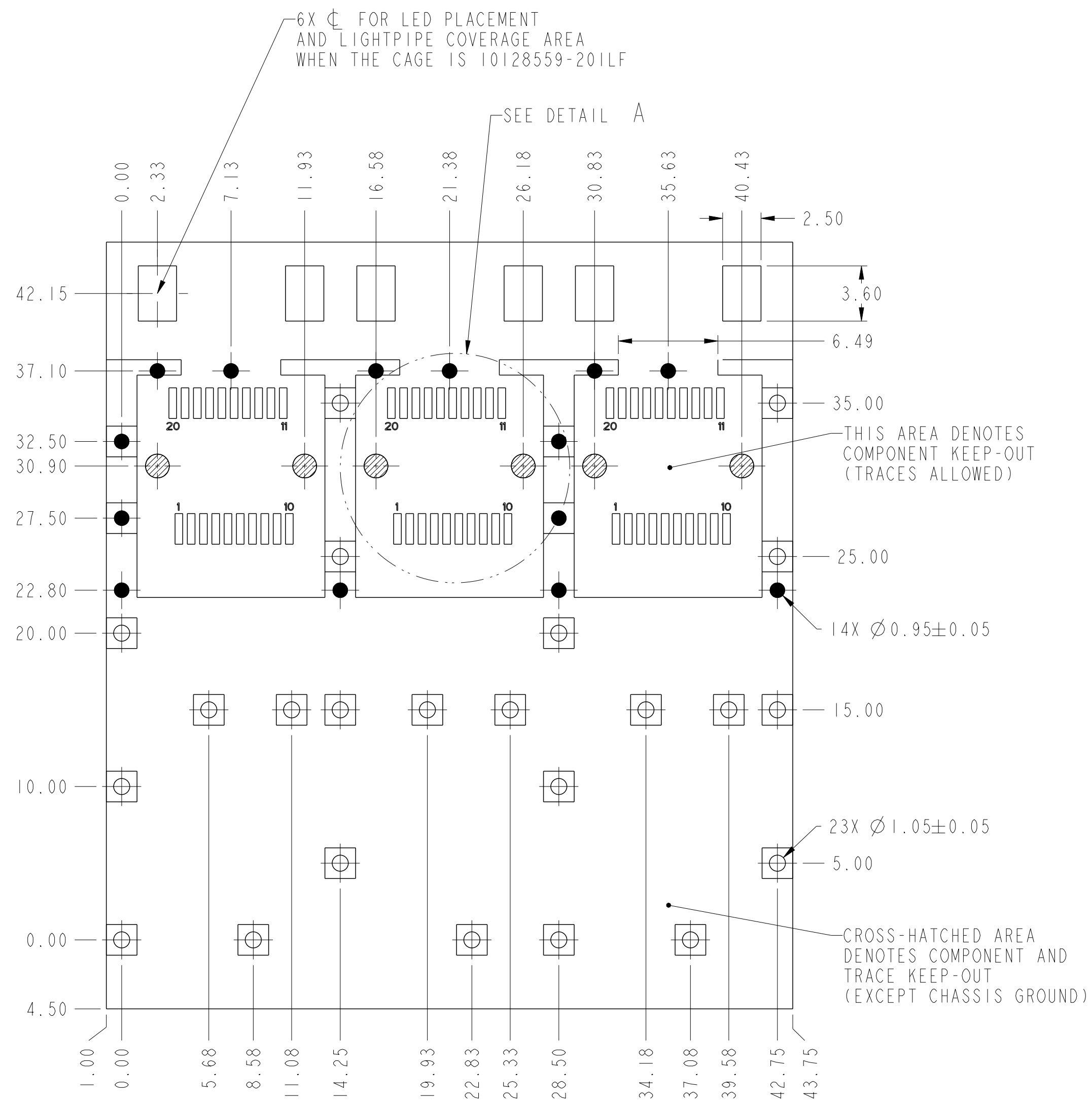
PCB LAYOUT
