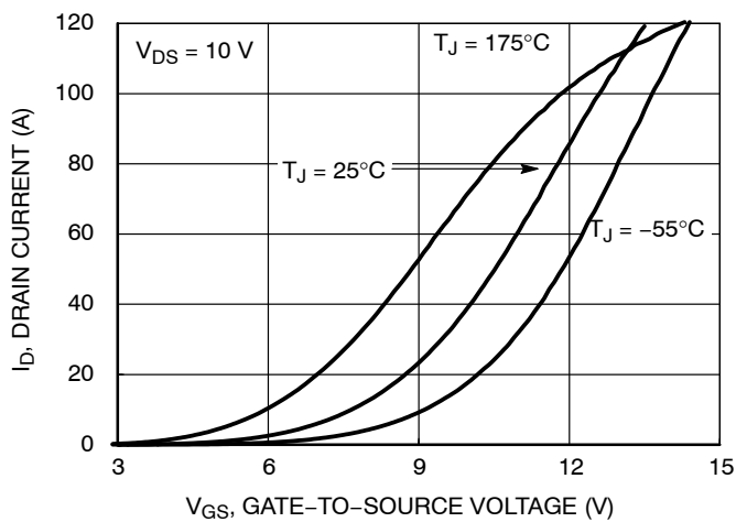
Figure 5. Transfer Characteristics
