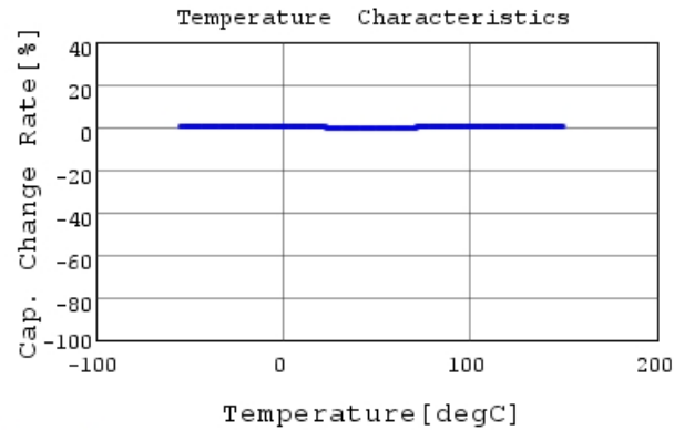
GJM0335G2A7R8WB01 C-Temp. capchange, DCOV, 1
