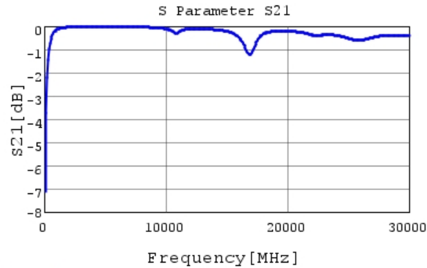
GJM0335G2A7R8WB01 S21 DCOV, 25degC
