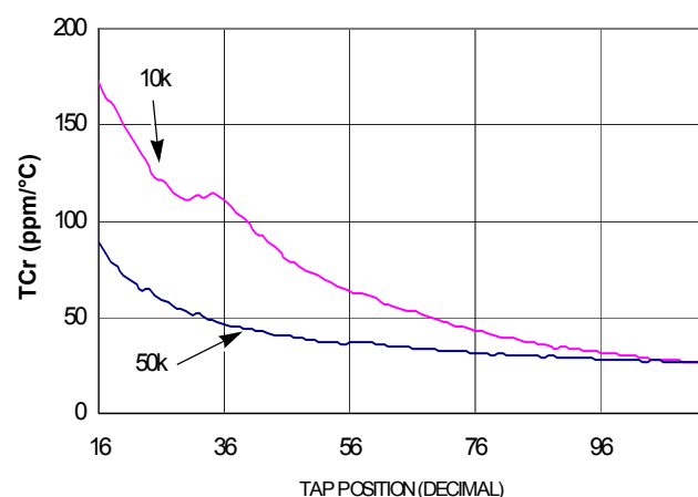
FIGURE 11. TC FOR RHEOSTAT MODE IN ppm
