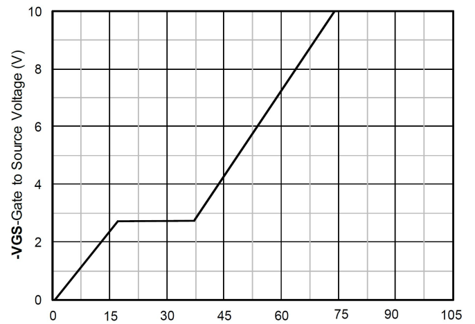
Gate Charge
