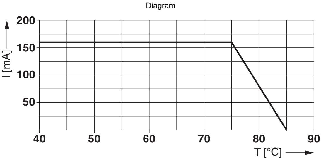
Derating curve at 55.2 V DC
