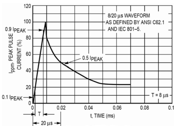
Figure 10. Pulse waveform
